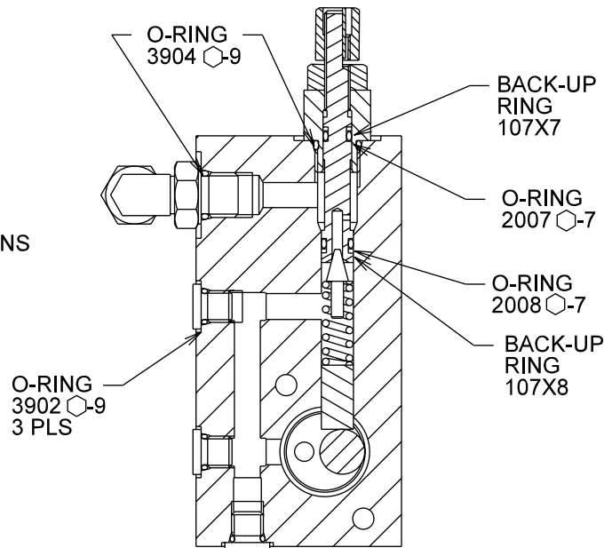
"ME" COMPENSATOR (REMOTE W/EXTERNAL SENSE) ITEM 63
